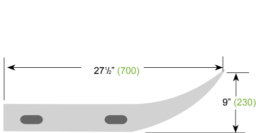
End Section (Flared)
