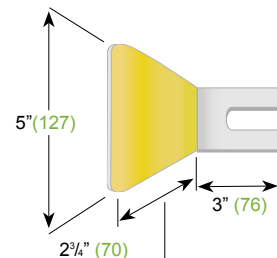
Reflectorized Washer
