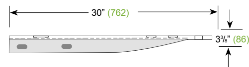
Terminal Connector Parapet
